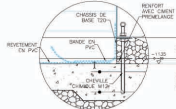
DETAIL "B1" ECHELLE 1:5
