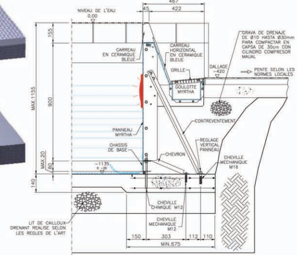
DETAIL "B" ECHELLE 1:10
