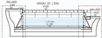
DETAIL "C" 4000 DETAIL "B"
